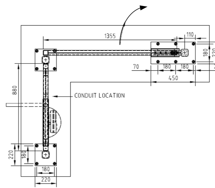
MRGE 4B-101 MRGE Right Hand Swing with Infill Drawing 3298-02 Rev 1
