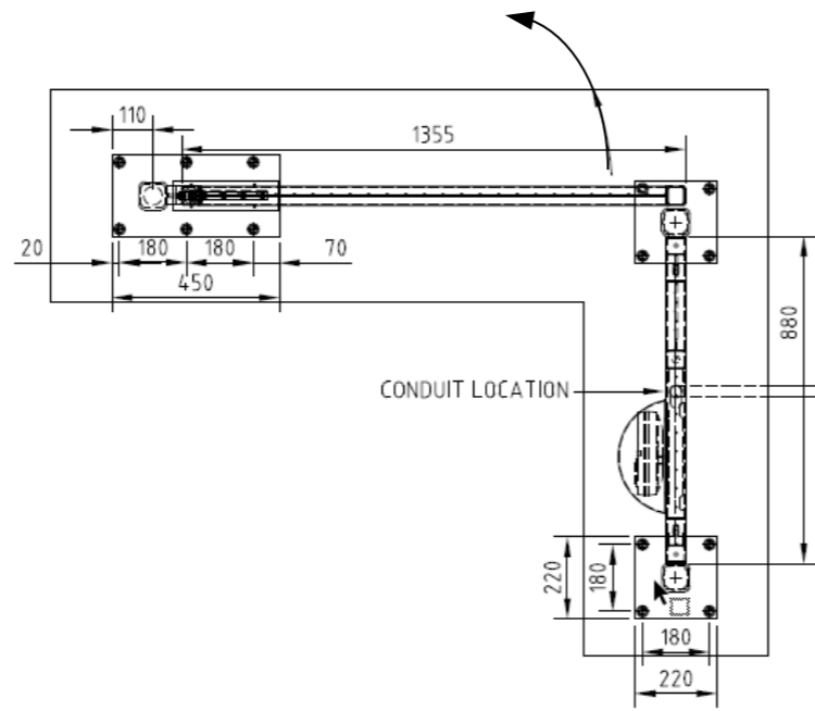
MRGE 4A-101 MRGE Left Hand Swing with Infill Drawing 3298-01 Rev 1
