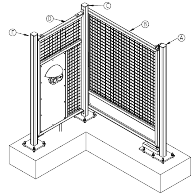
MRGE 4B-101 MRGE Right Hand Swing with Infill Drawing 3298-02 Rev 1
