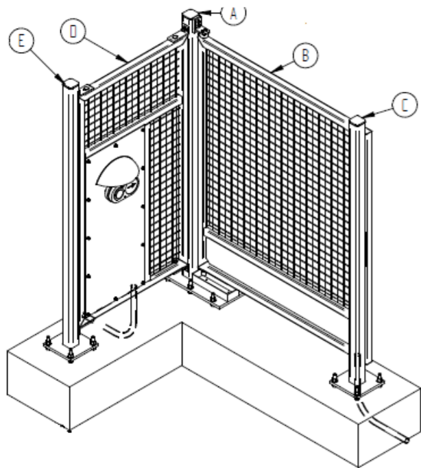
MRGE 4A-101S MRGE Left Hand Swing with Infill Drawing 3410-02 Rev 1
