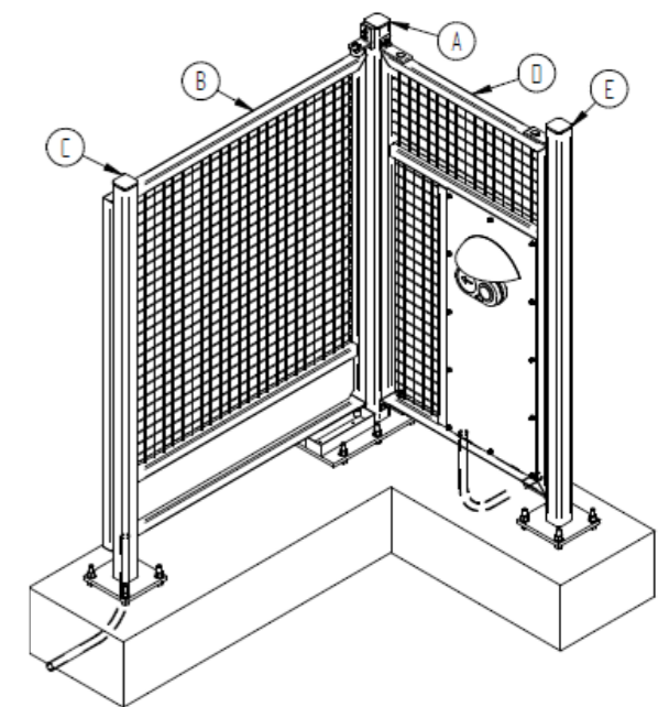
MRGE 4B-101S MRGE Right Hand Swing with Infill Drawing 3410-01 Rev 1
