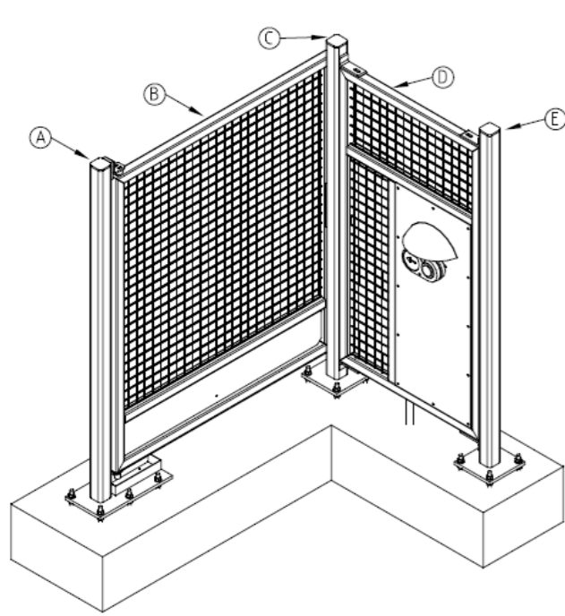
MRGE 4A-101 MRGE Left Hand Swing with Infill Drawing 3298-01 Rev 1
