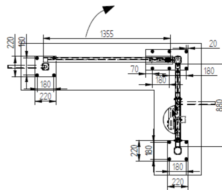
MRGE 4B-101S MRGE Right Hand Swing with Infill Drawing 3410-01 Rev 1
